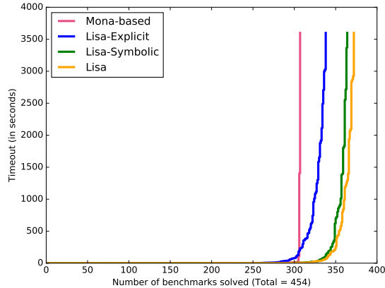
Figure 1: DFA construction. Cactus plot indicating number of benchmarks each tool can solve for a given timeout.
