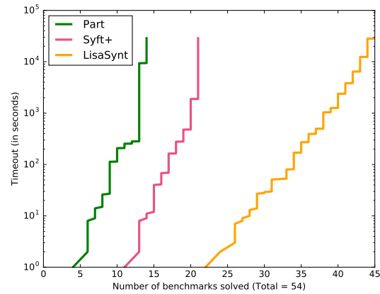
Figure 5: Synthesis. Cactus plot (non-random benchmarks).
